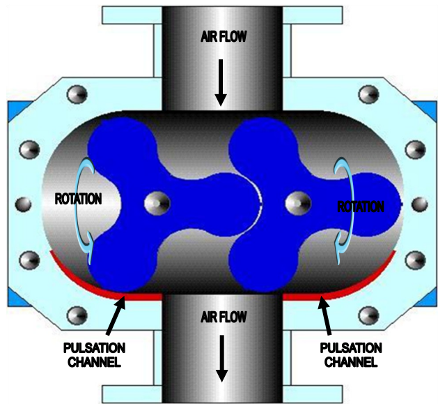
Tri-Lobe with Pulsation Control
