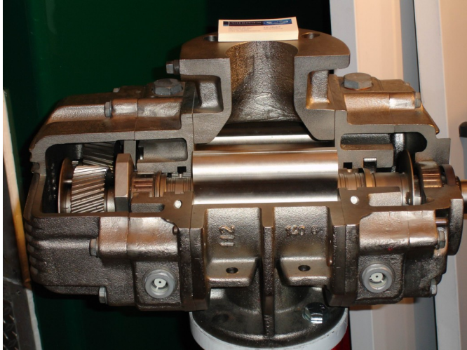
Trilobe Blower Cutaway
